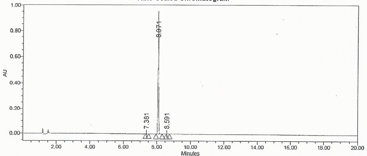
Auto-Scaled Chromatogram
